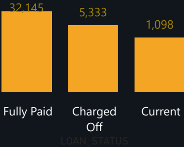
Loan Application
